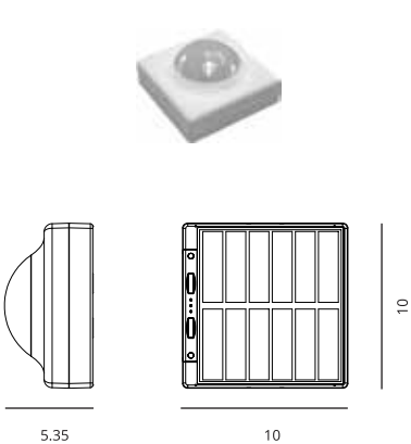
Solar Hybrid Module S (Pose 1, 2, 3) Item Code : LP6532
